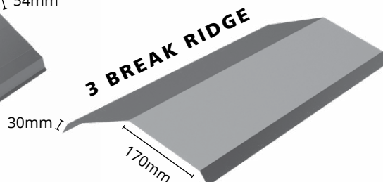
BARGE CAPPING
