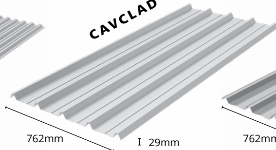
TRIMDECK
